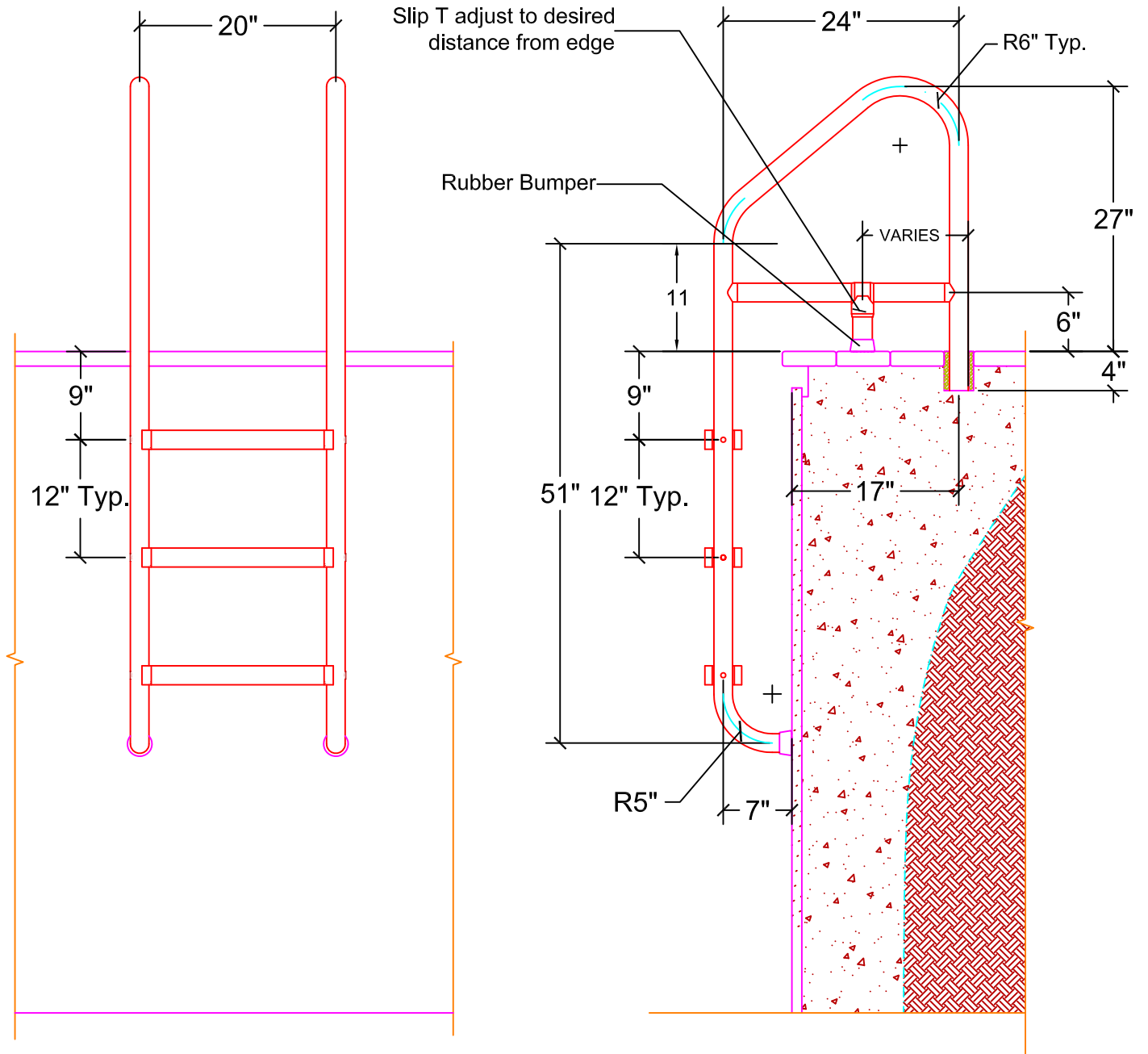
CBL-324-3S
