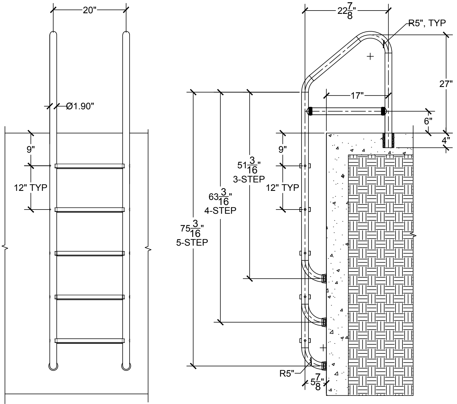
CBL-324-3S/4S/5S
